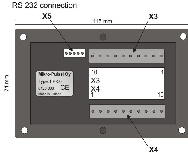
Control unit from behind
